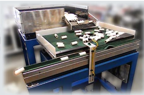
FLEX-FEEDERS VERSATILE VIBRATORY RE-CIRCULATOR FOR ROBOT / VISION LOADING SYSTEMS
